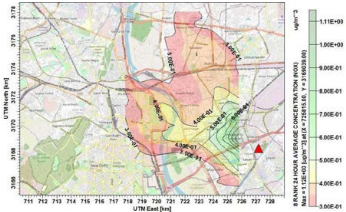
Figure 23: Isopleth of daily average GLC of NO x around Ghazipur WtE plant.
