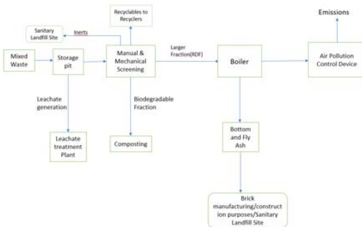
Figure 1: Process description diagram of Waste to Energy Plant
