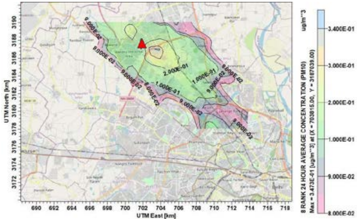
Figure 13: Isopleth of daily average GLC of PM around Bawana WtE plant.
