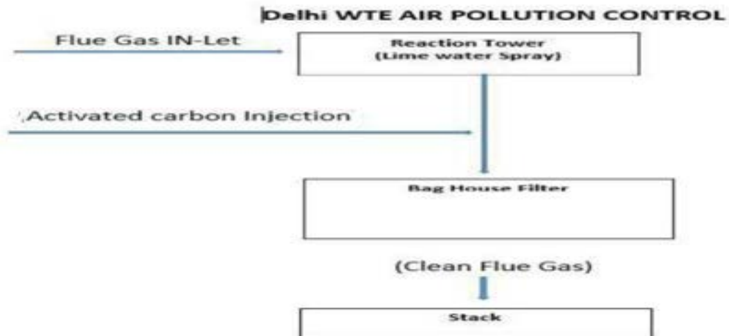
Figure: Flow diagram of APCD in Bawana WtE plant
