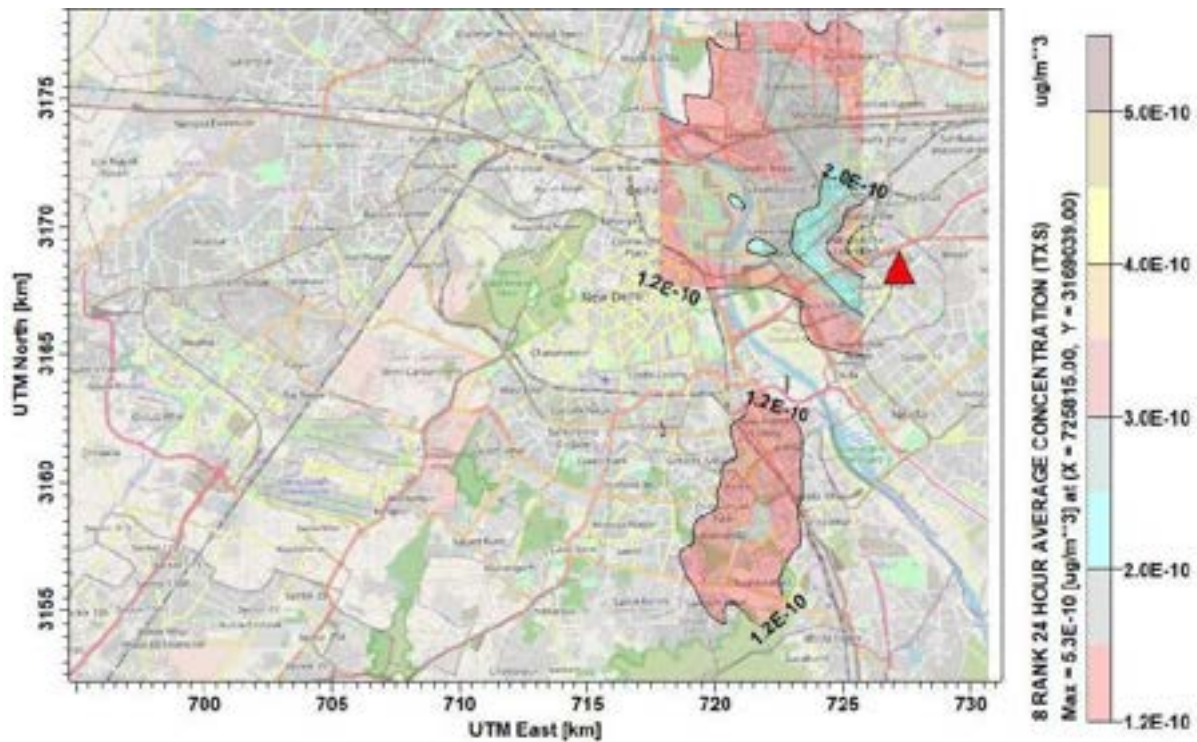
Figure 27: Isopleth of daily average GLC of Dioxin around Ghazipur WtE plant.
