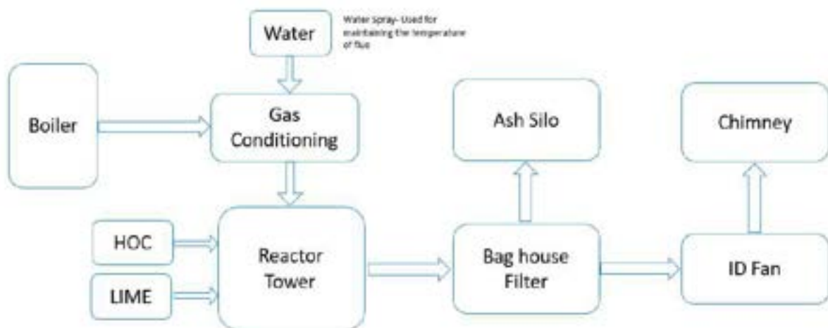
Figure: Flow diagram of APCD in Tehkhand WtE plant
