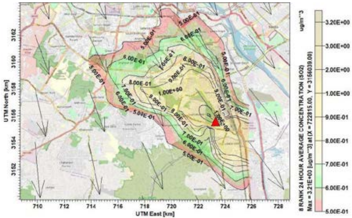
Figure 33: Isopleth of daily average GLC of \text{SO}_2 around Tehkhand WtE plant.
