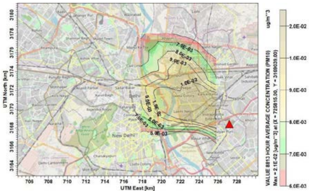
Figure 22: Isopleth of annual average GLC of PM around Ghazipur WtE plant.
