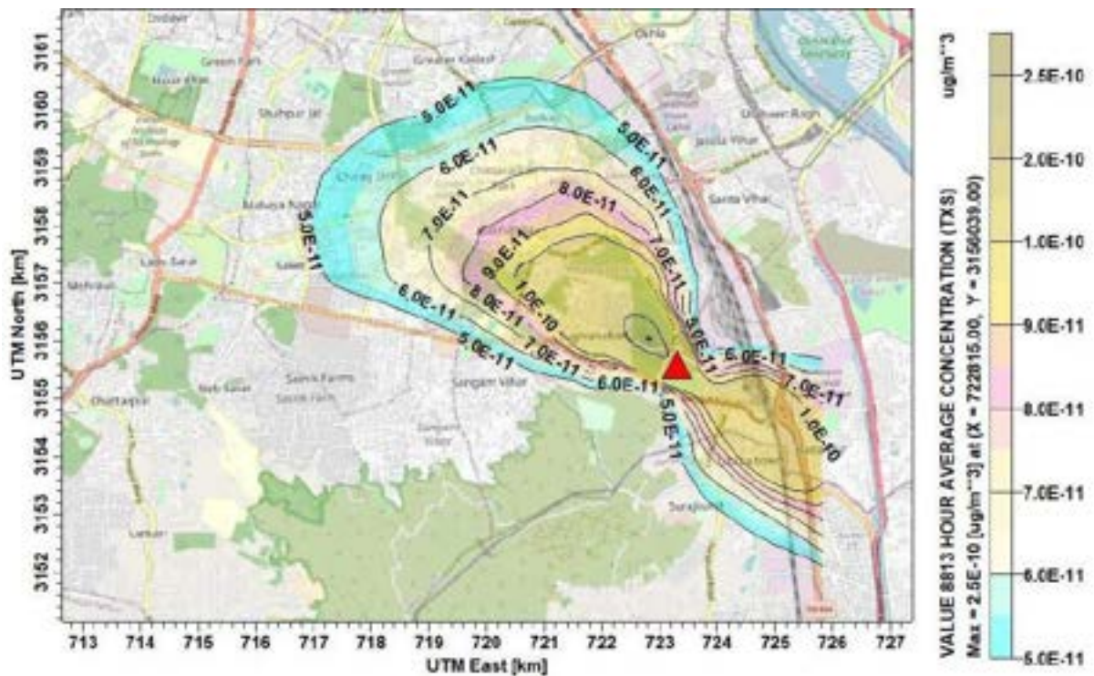
Figure 36: Isopleth of annual average GLC of Dioxin around Ghazipur WtE plant.
