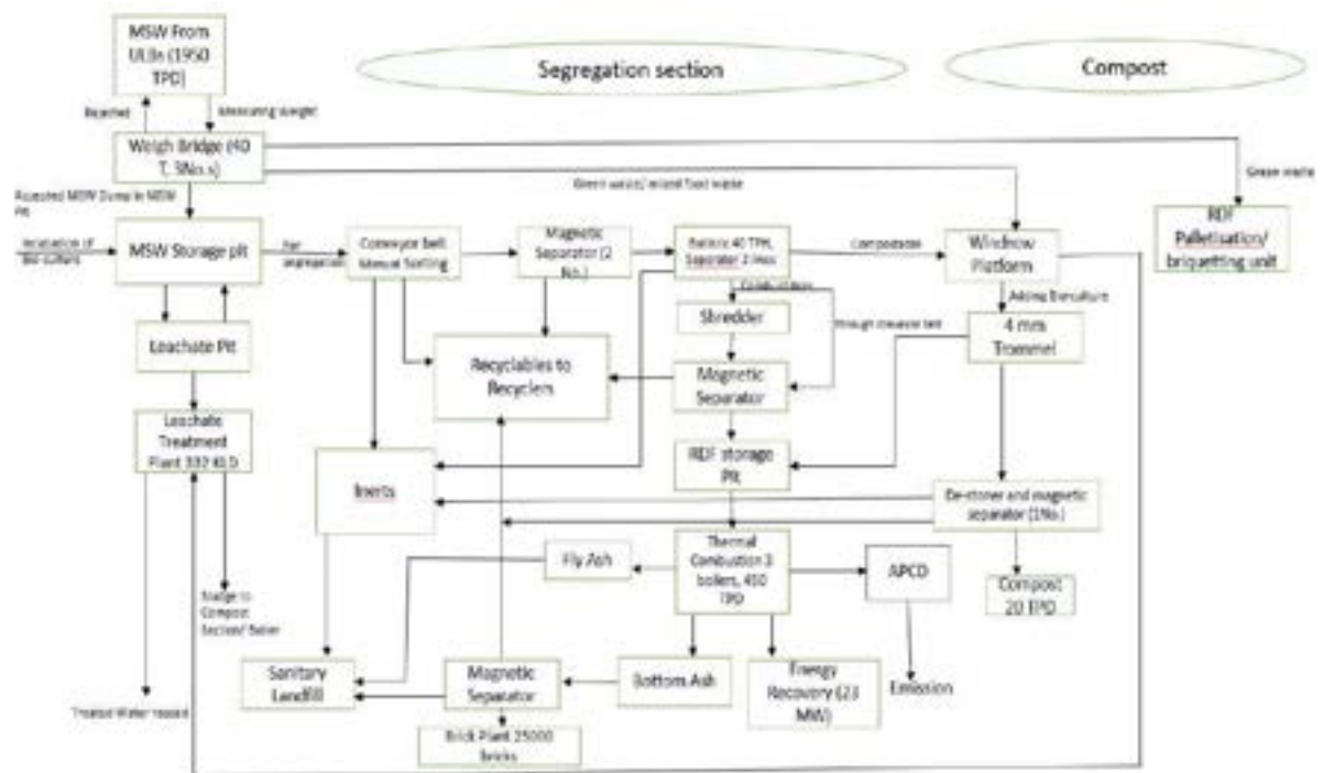
Figure: Process flow diagram of Okhla WtE
