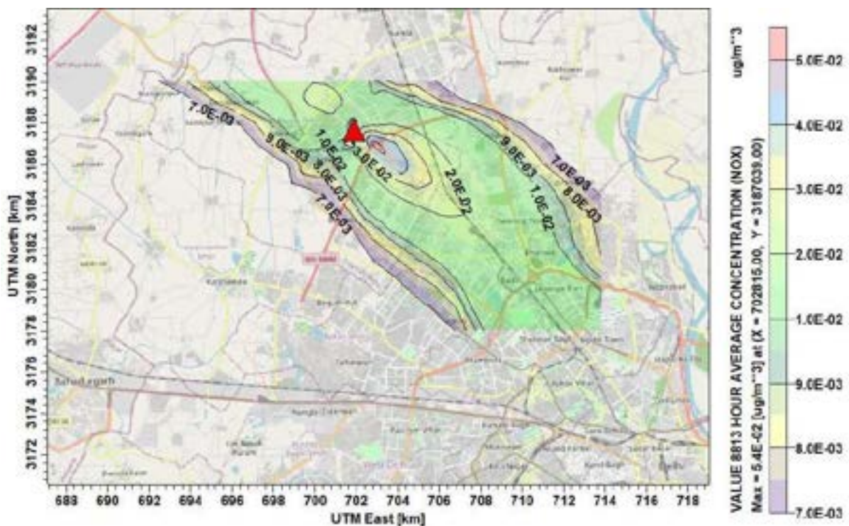
Figure 16: Isopleth of annual average GLC of NOx around Bawana WtE plant.
