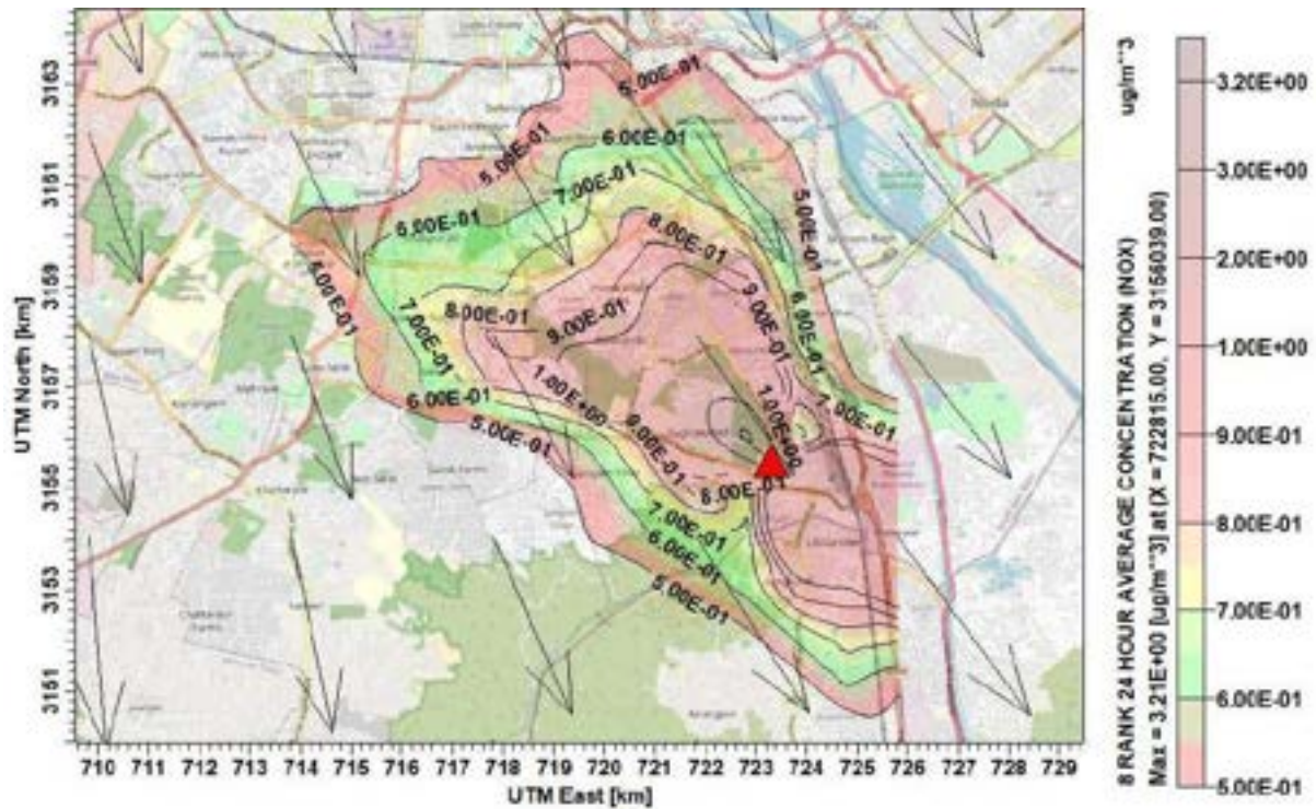
Figure 31: Isopleth of daily average GLC of NO x around Tehkhand WtE plant.
