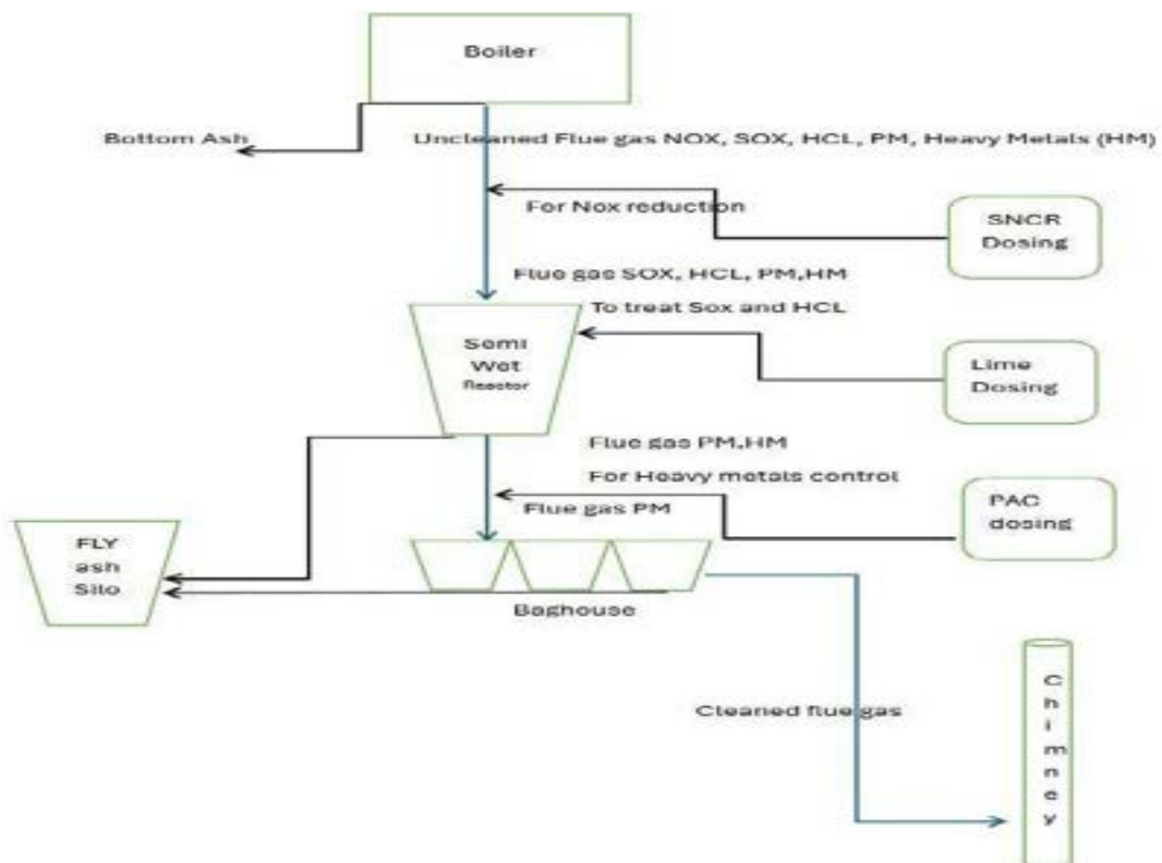
Figure: Flow diagram of APCD in Ghazipur WtE plant
