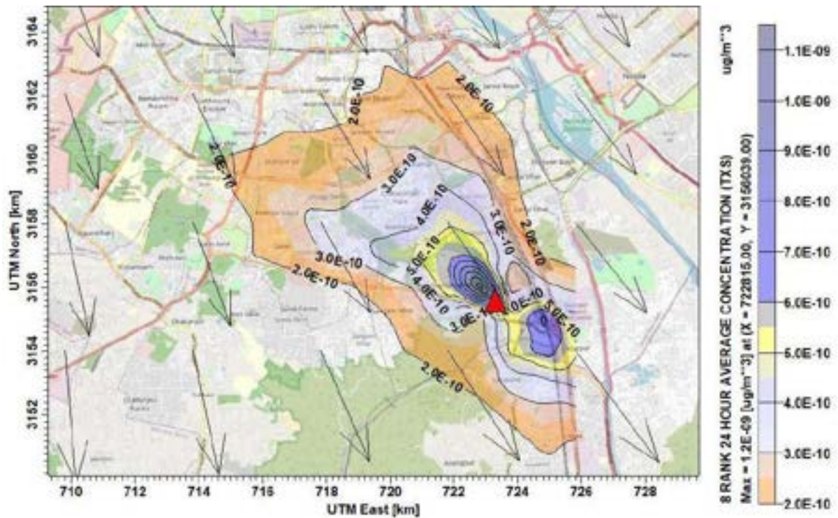
Figure 35: Isopleth of daily average GLC of Dioxin around Tehkhand WtE plant.
