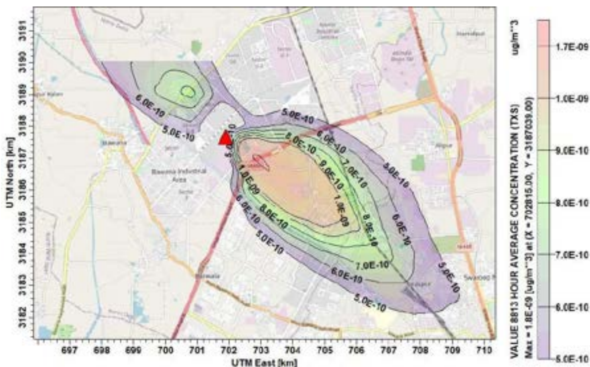
Fig. 20: Isopleth of annual average GLC of Dioxin around Bawana WtE plant.
