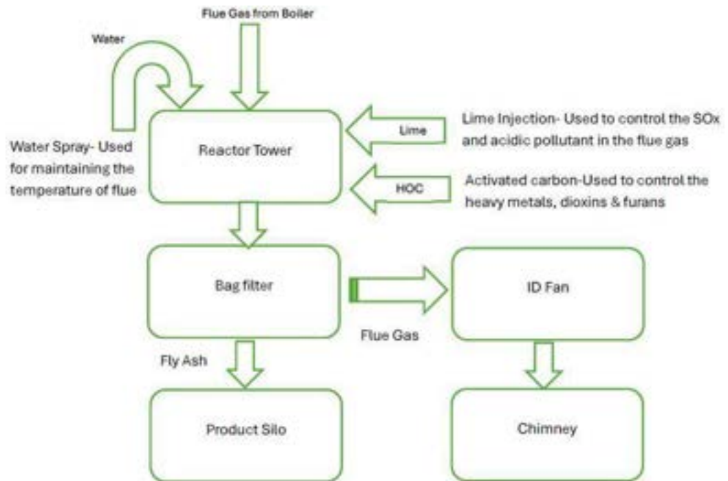
Figure: Flow diagram of APCD in Okhla WtE plant
