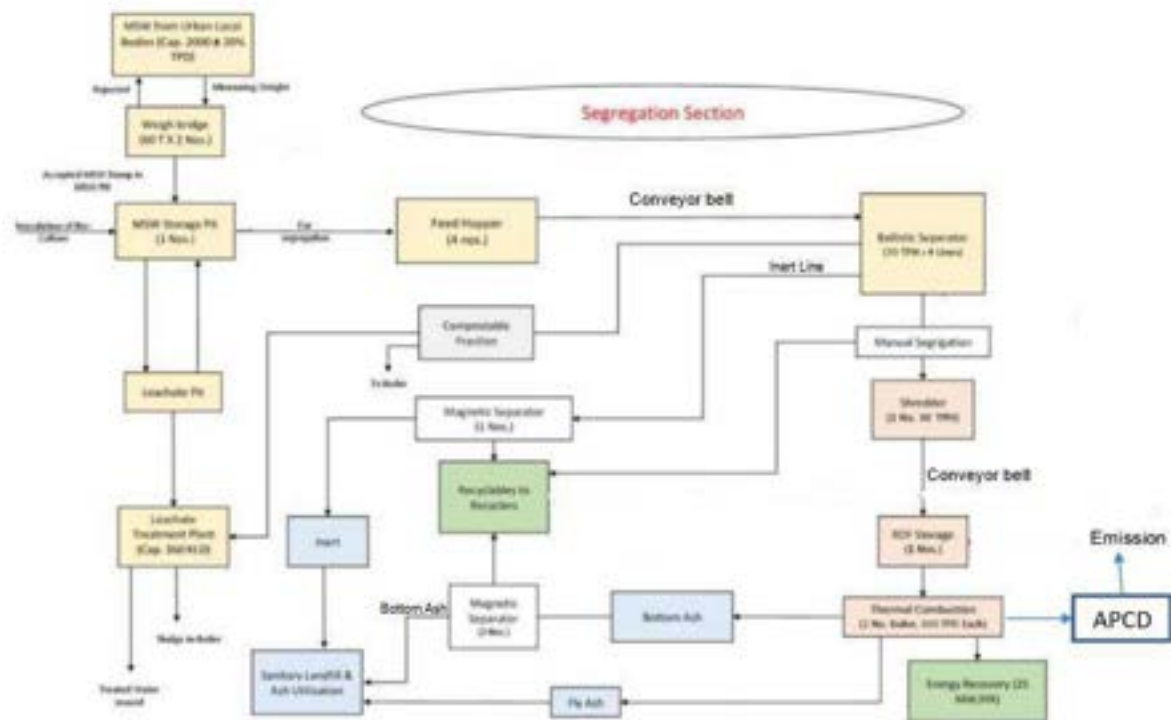
Figure: Process flow diagram of Tehkhand WtE
