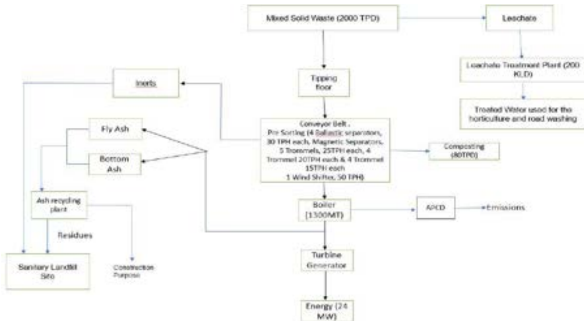
Figure: Process flow diagram of Bawana WtE
