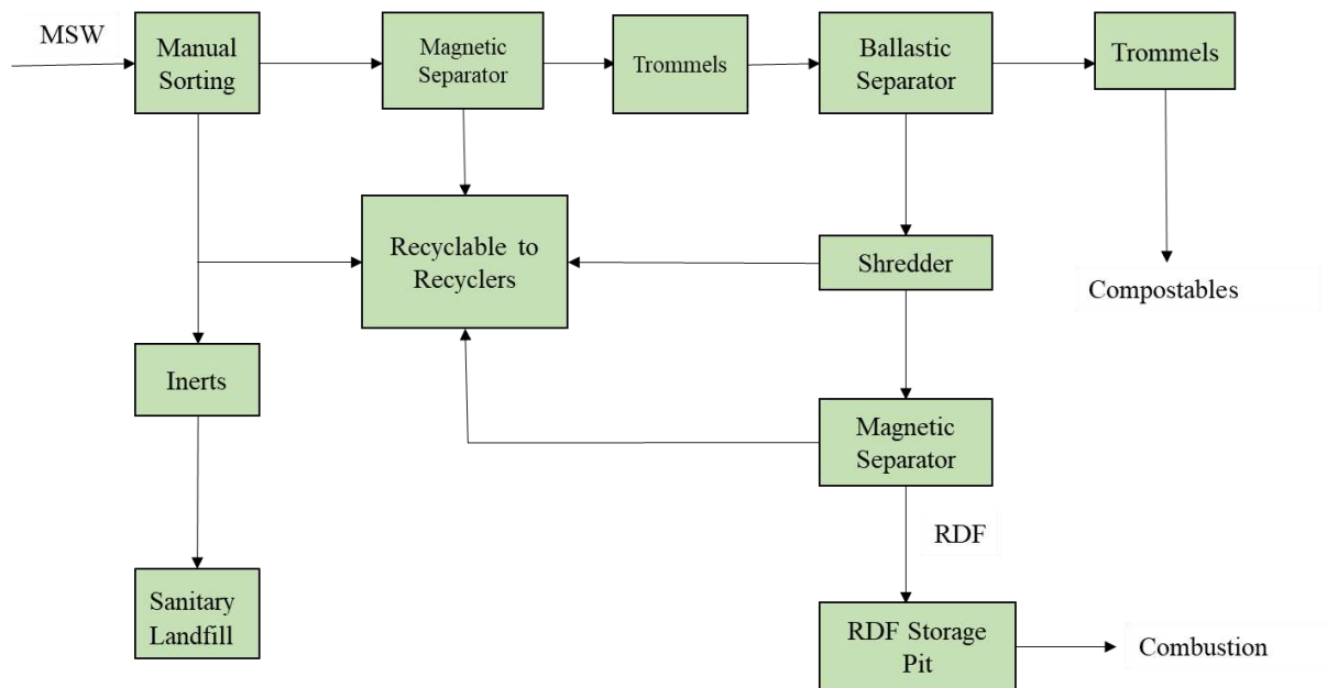
Figure 11: Segregation steps in WtE facility
