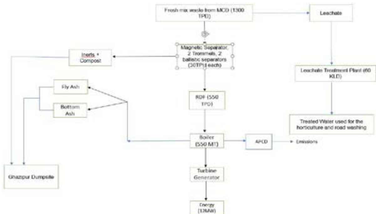
Figure: Process flow diagram of Ghazipur WtE
